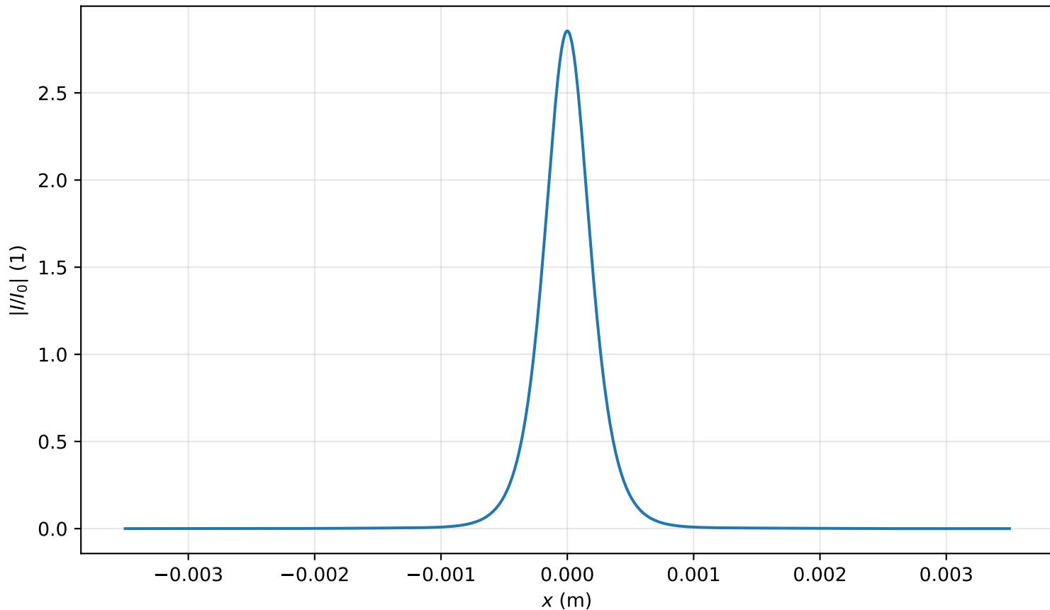
Intensity profile I(x, y = 0, z = 3.344m)/I_0 , P_{in}=1.0P_{cr} , artificial time
